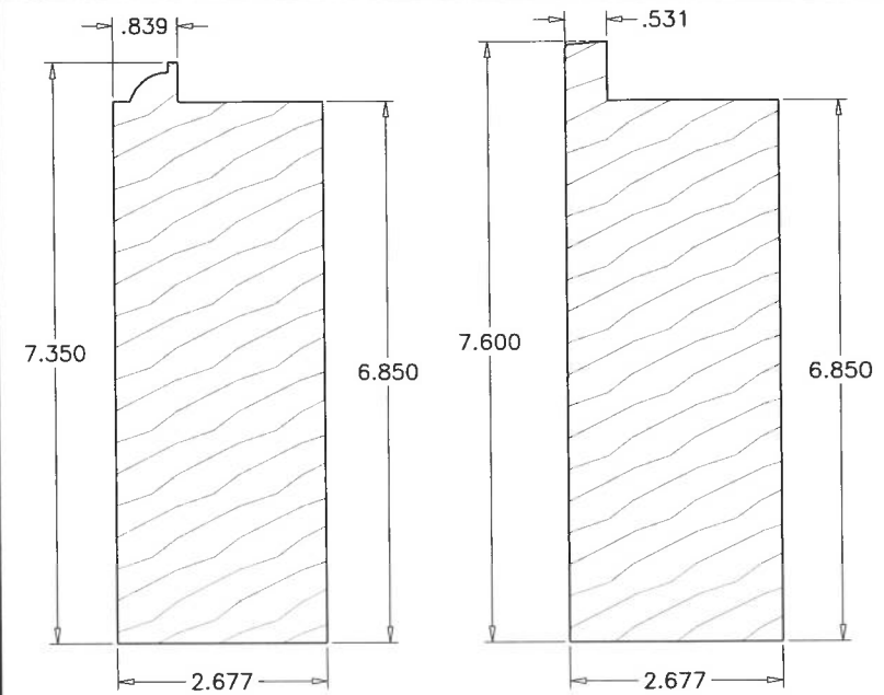
2 RAIL
