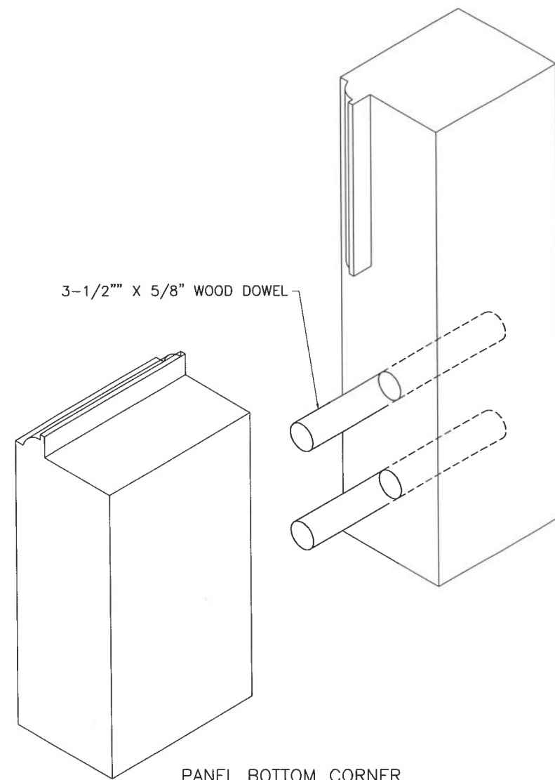
PANEL BOTTOM CORNER
