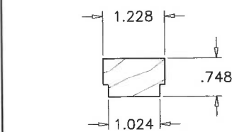
13 ANCHOR COVER
