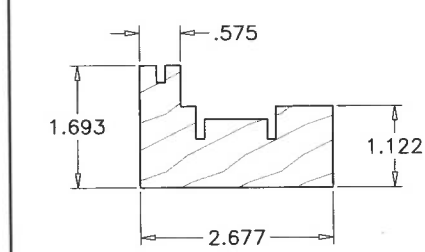
14 FRAME
