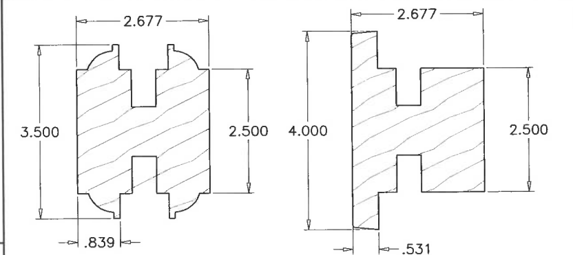
6 INTERMEDIATE STILE
