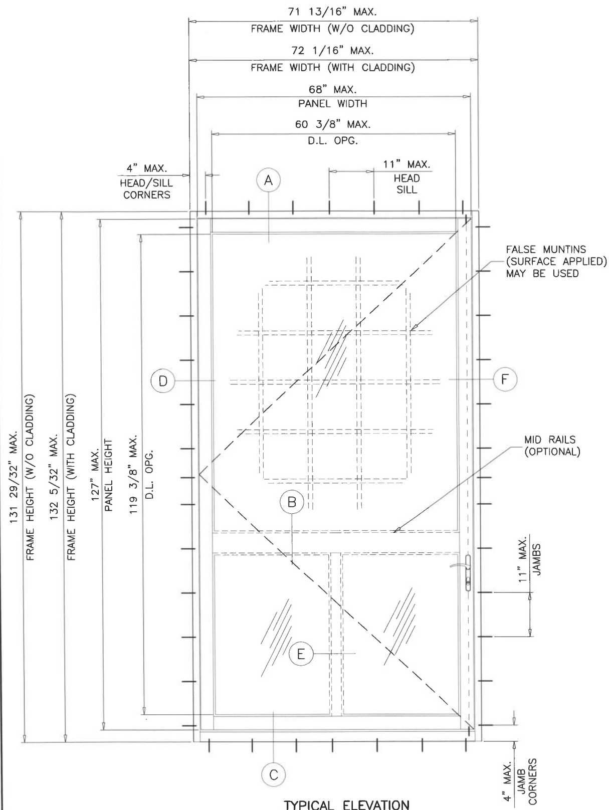
TYPICAL ELEVATION
