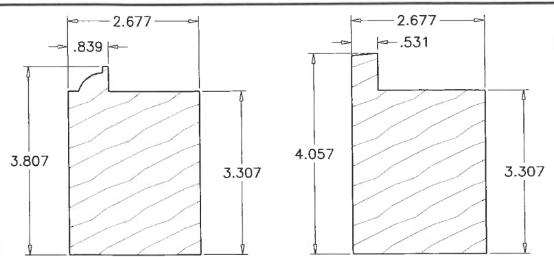
1 STILE/RAIL
