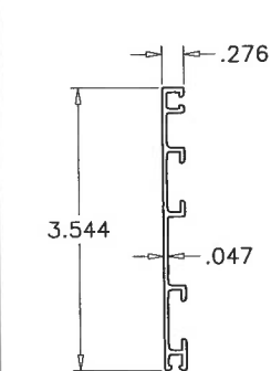
21 STILE/RAIL CLADDING
