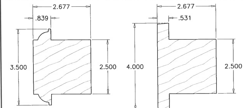
3 INTERMEDIATE STILE
