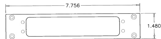
25 TOP PIVOT SUPPORT PLATE
