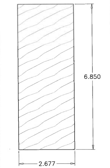
9 INTERMEDIATE STILE/RAIL
