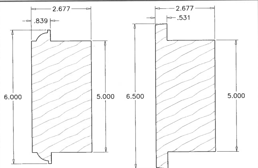
4 INTERMEDIATE STILE/RAIL
