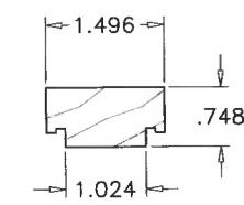
15 ANCHOR COVER
