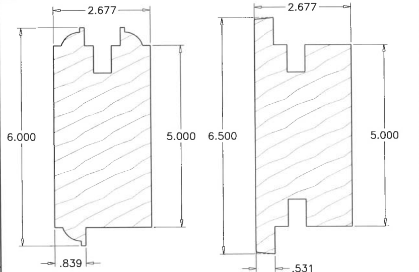
5 INTERMEDIATE STILE/RAIL
