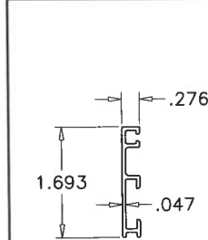
12 FRAME
