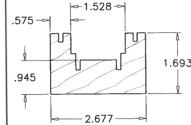
14 FRAME
