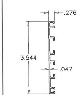
22 INT. STILE/RAIL CLADDING
